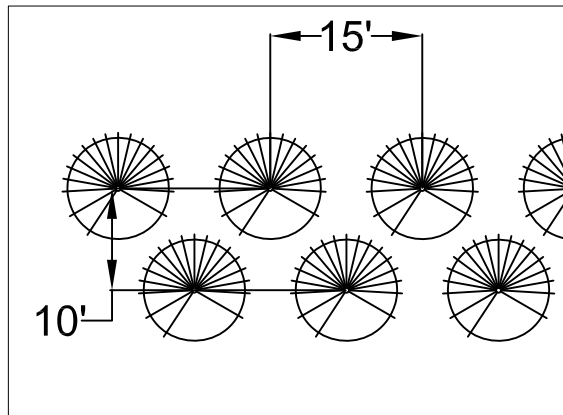
DETAILED PLAN VIEW OF TYPICAL PLANT SPACING
